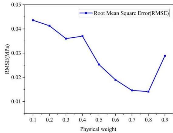
Fig. 7. Performance of PDF under different physical weights.
