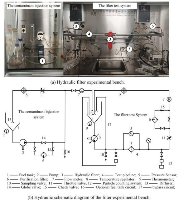
Fig. 3. Hydraulic filter degradation experiment bench.
