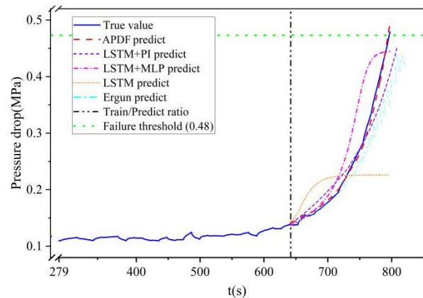
Fig. 5. Performance of different prediction models. The figure only displays the data from the degradation phase, as the data from the healthy phase was removed since it is not involved in training and prediction.
