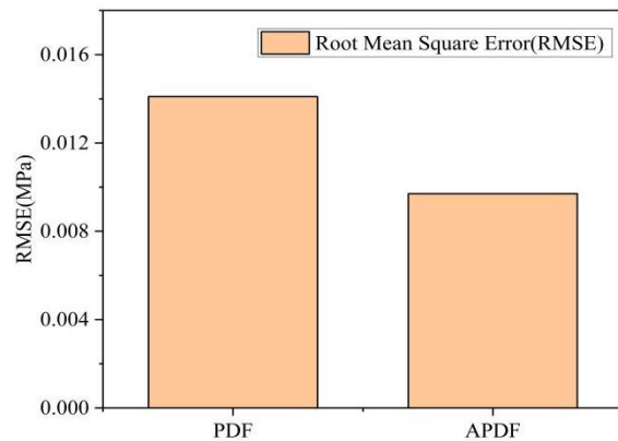
Fig. 8. Comparison of predictive performance between best-performing fixed-weight PDF and APDF.
