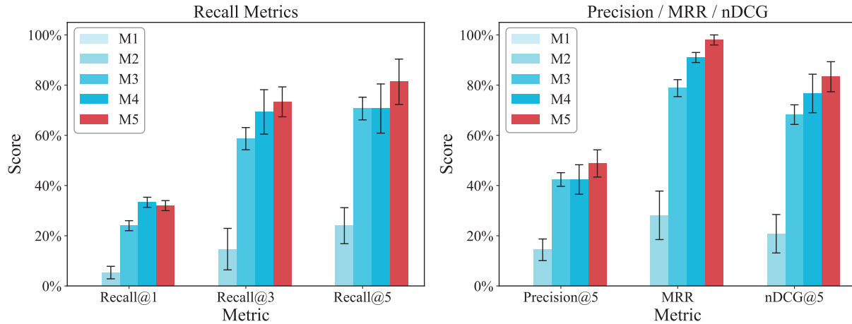
Fig. 4. Comparison of retrieval performance metrics across different methods.
