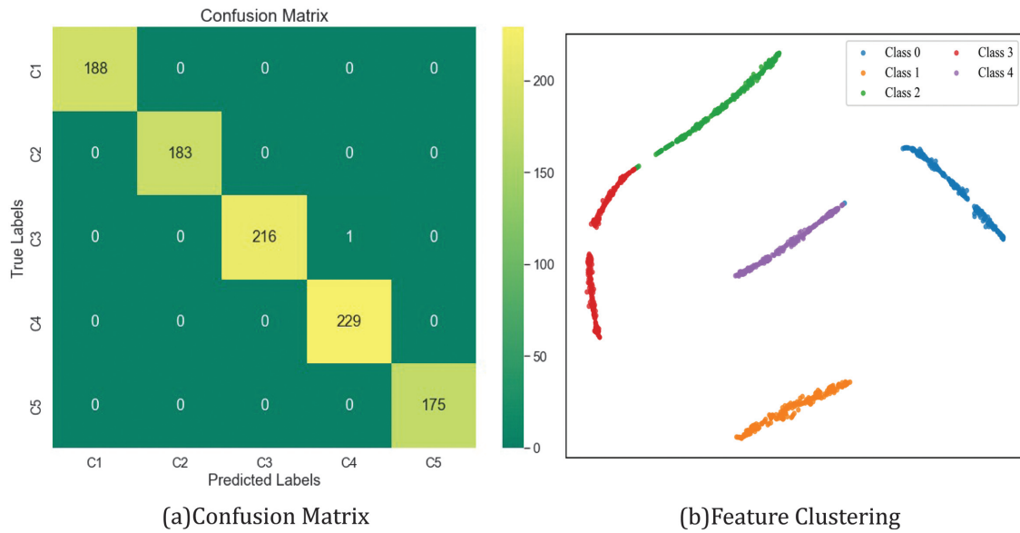
Fig. 12. Confusion matrix and feature clustering on the Southeast University Dataset.
