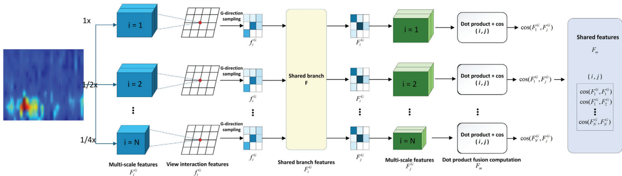
Fig. 4. Scaled dot-product attention mechanism.
