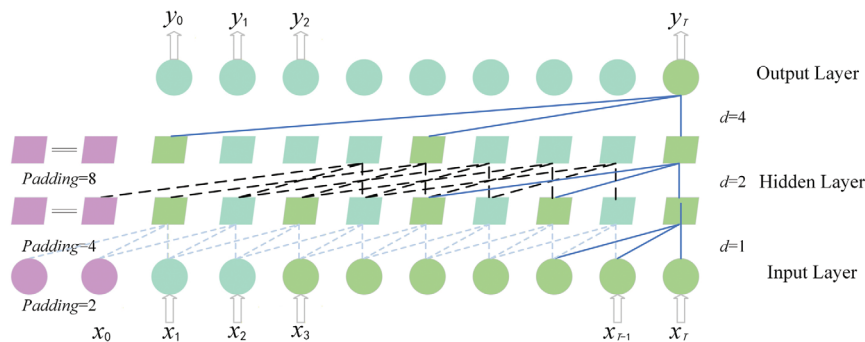
Fig. 1. Expanded causal convolution structure.
