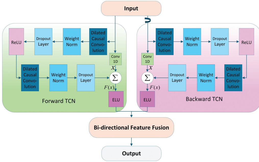
Fig. 2. BiTCN feature extraction process.
