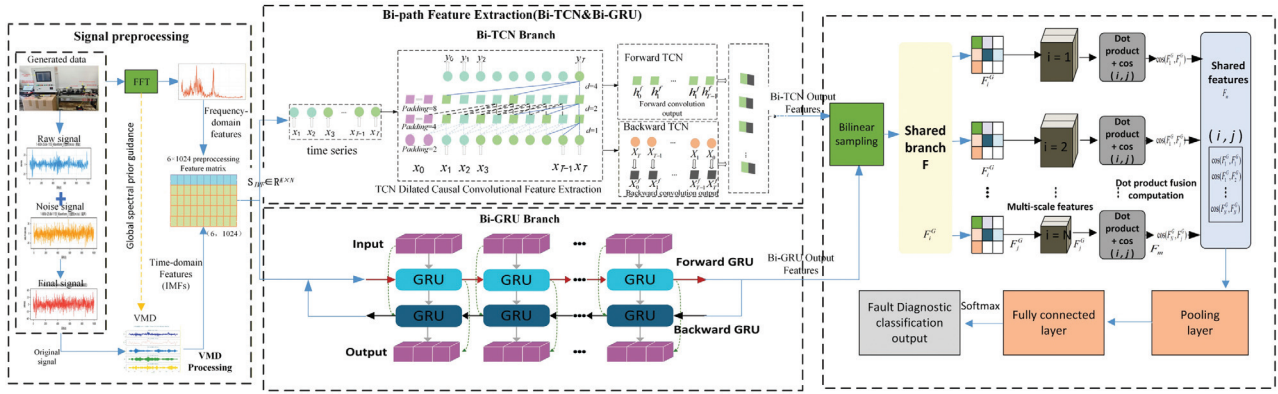
Fig. 5. Full model flowchart.
