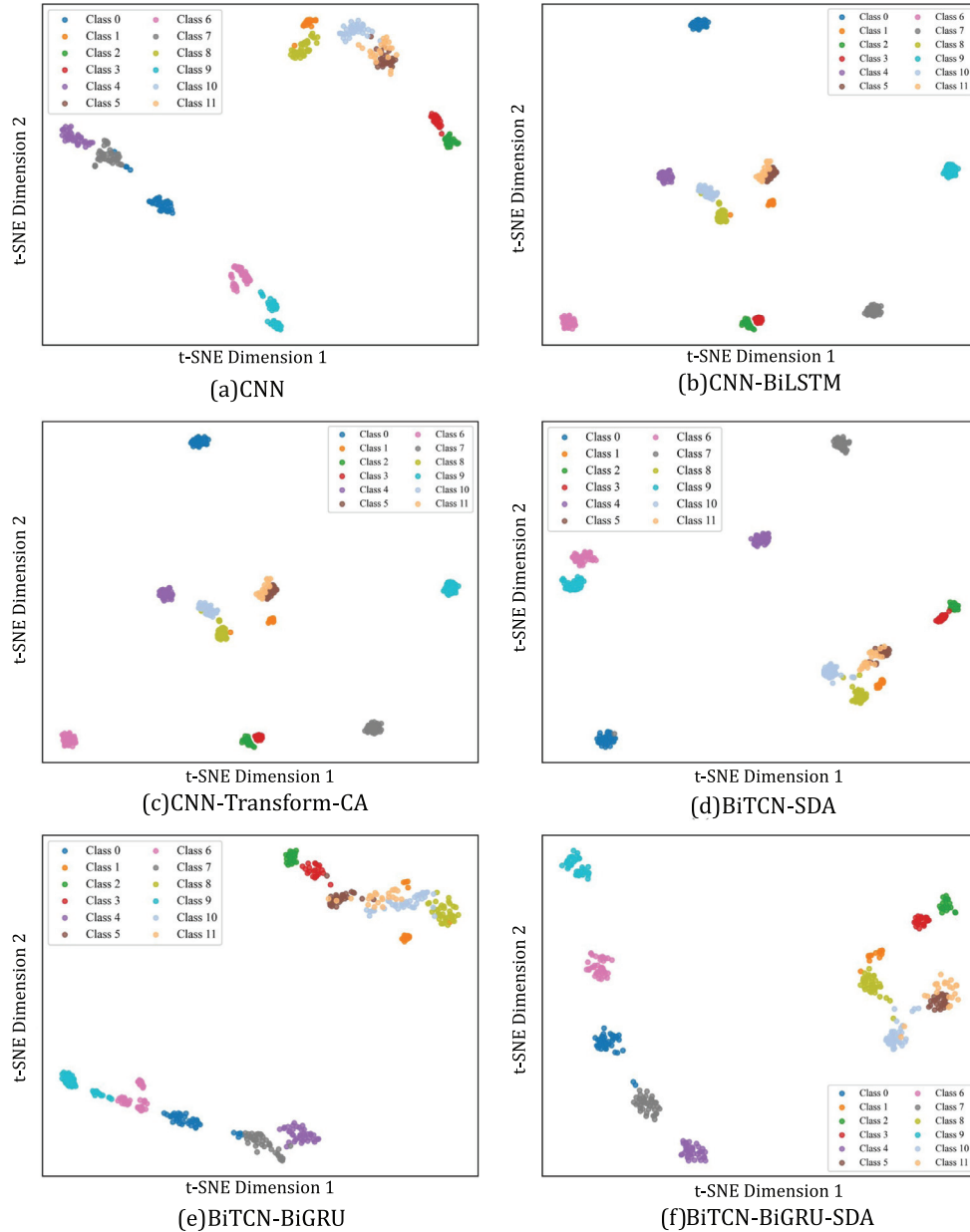
Fig. 11. t-SNE feature clustering results for different models.
