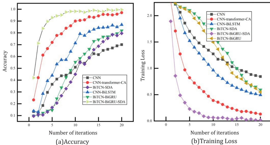
Fig. 9. Training accuracy and loss curves.
