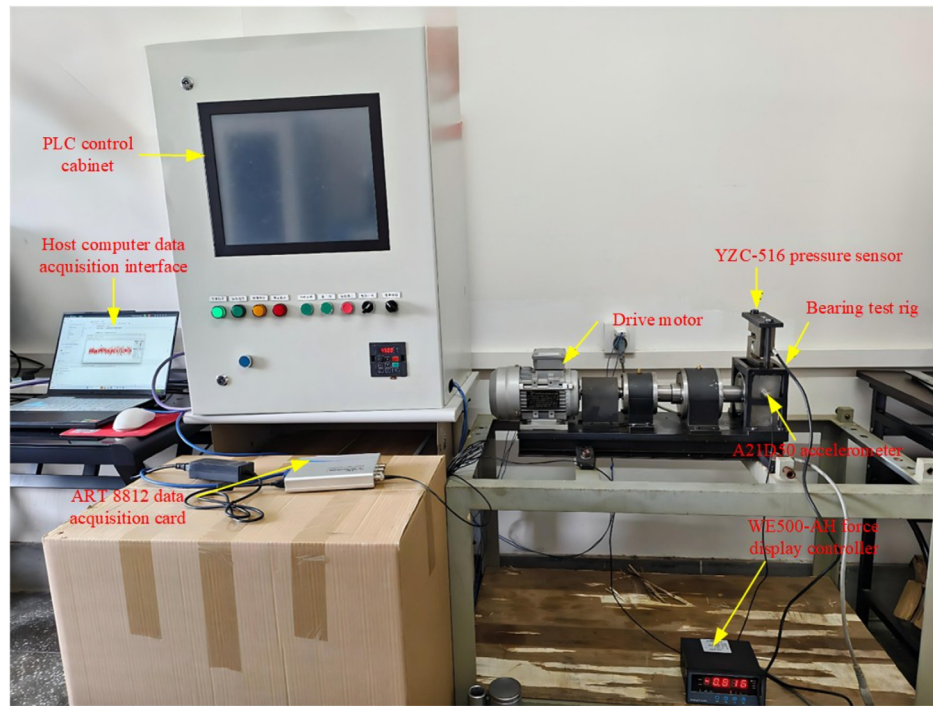
Fig. 6. Bearing testing machine.
