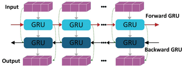
Fig. 3. BiGRU feature extraction process.
