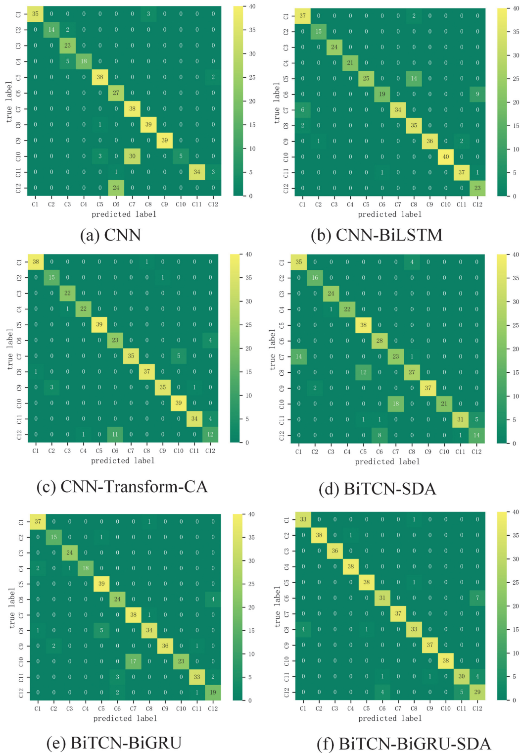
Fig. 10. Confusion matrices for different models.
