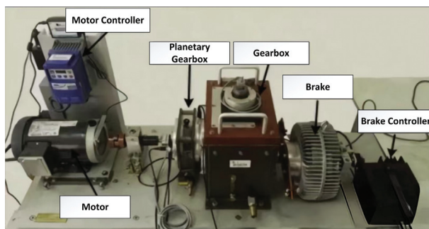
Fig. 8. Bearing testing platform.
