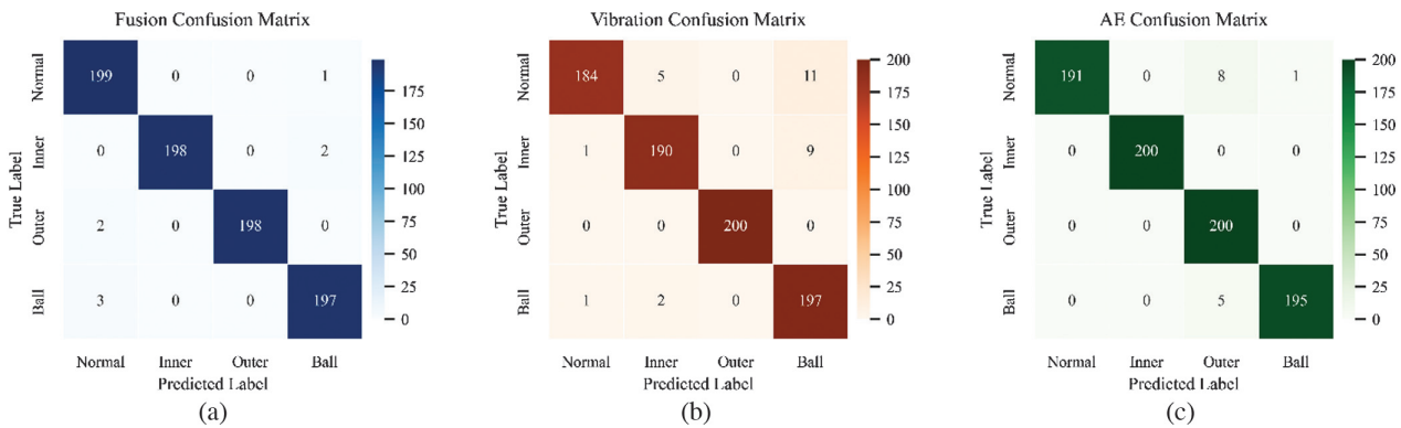
Fig. 2. Representative confusion matrices under the strict source-group-disjoint protocol: (a) vibration + AE fusion, (b) vibration-only, and (c) AE-only.
