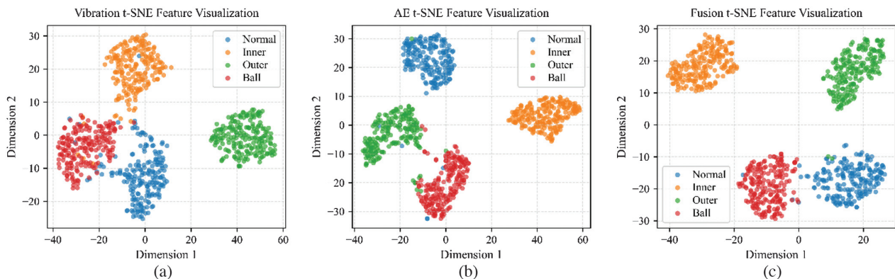
Fig. 3. t-SNE visualization of learned features: (a) vibration-only, (b) AE-only, and (c) vibration + AE fusion.
