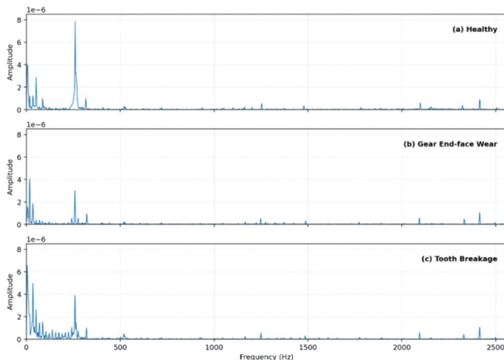
Fig. 3 . Pressure spectra under different fault conditions.
