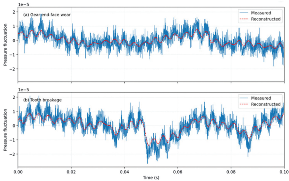
Fig. 4. Time-domain comparison between measured and reconstructed outlet pressure signals.
