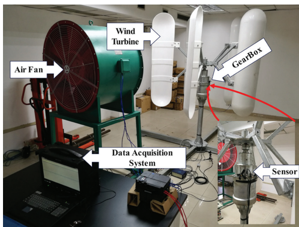
Fig. 4. Experimental setup of the wind turbine system.
