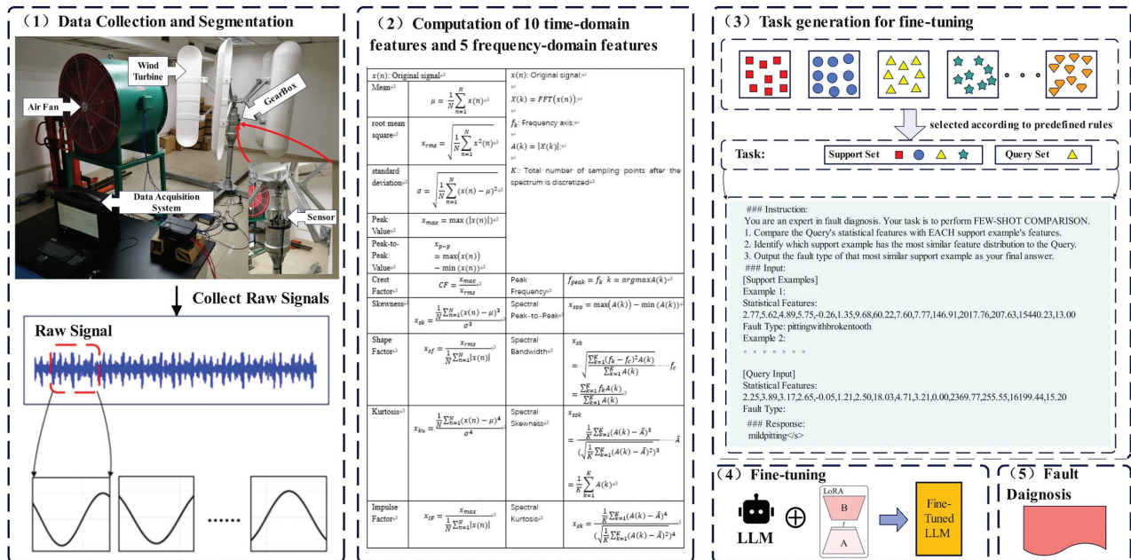
Fig. 6. Framework flowchart.
