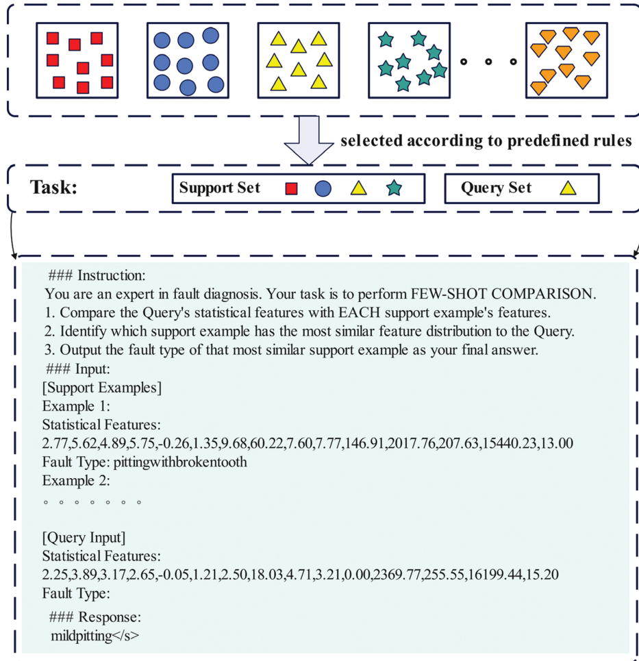
Fig. 1. Task-based fault diagnosis dataset.
