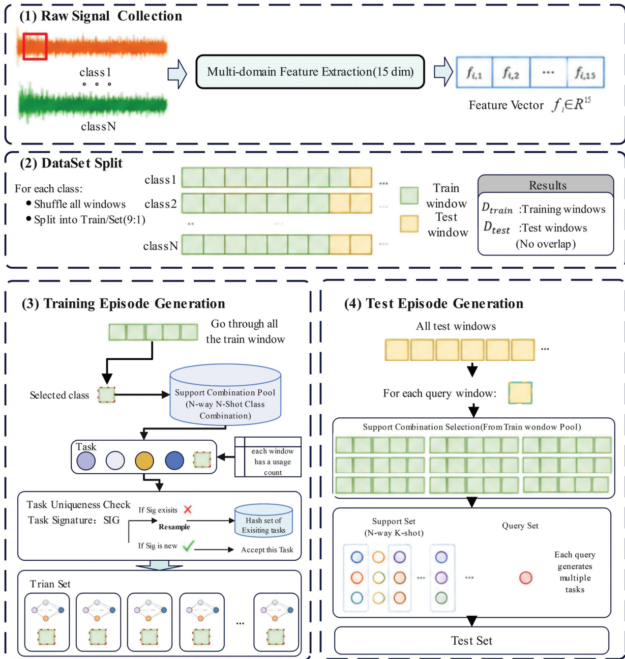
Fig. 2. Dataset construction flowchart.
