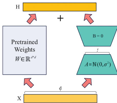
Fig. 3. LoRA fine-tuning process.
