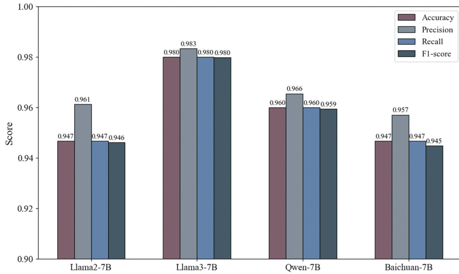
Fig. 7. Performance metric.
