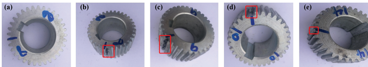
Fig. 5. Fault details: (a) healthy; (b) light pitting; (c) medium pitting; (d) partial tooth breakage; (e) 0.3 mm × 0.5 mm Worn.
