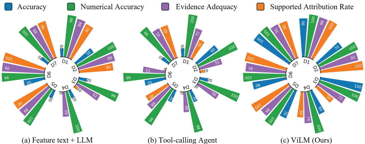
Fig. 5. Dataset-wise performance comparison of different diagnostic methods.
