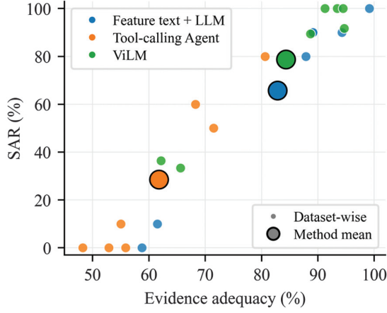
Fig. 6. Dataset-wise evidence reliability comparison.
