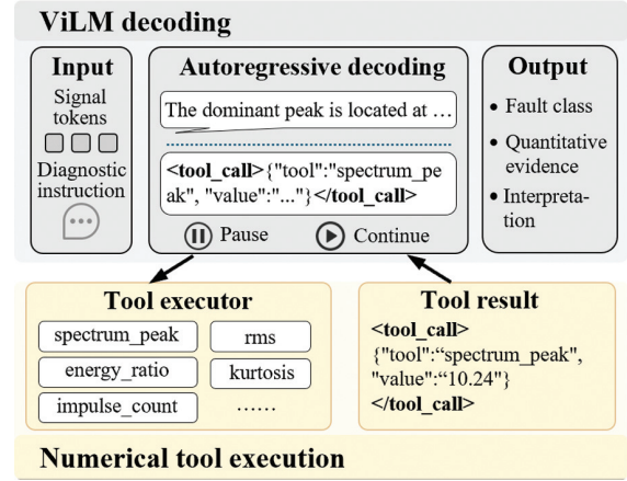
Fig. 4. Structured tool decoding process.
