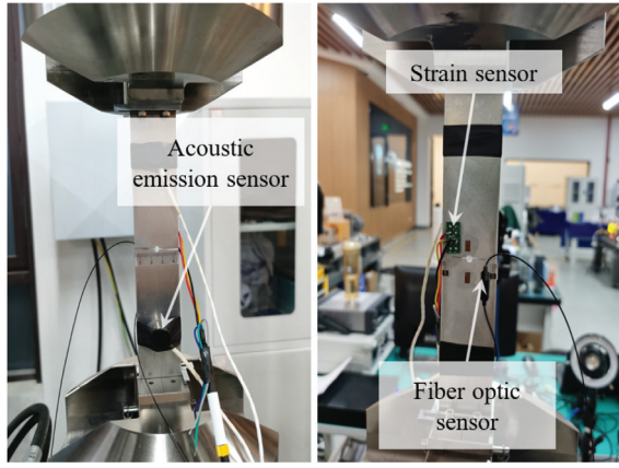
Fig. 6. Experimental 7050-aluminum center-hole coupon and acoustic-emission, strain-gauge, and Fibre Bragg Grating sensor arrangement.
