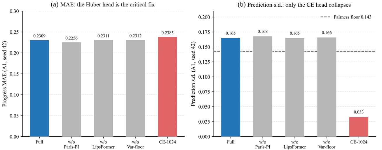
Fig. 10. Ablation of four design choices on scenario A1, seed 42: progress mean absolute error (a) and prediction standard deviation (b). Only the cross-entropy head collapses the prediction variance below the fairness floor.
