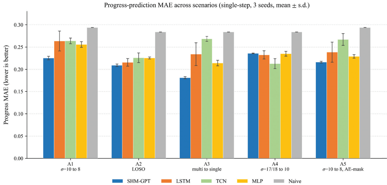
Fig. 7. Mean absolute error across scenarios with three-seed error bars.
