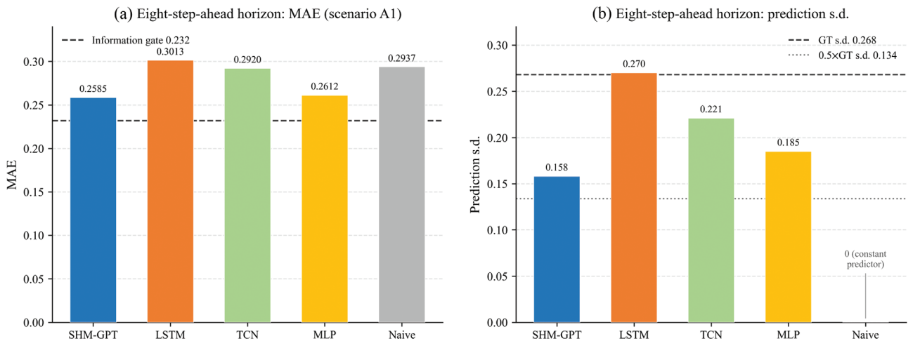
Fig. 11. Eight-step-ahead horizon stress test on scenario A1, seed 42: mean absolute error (a) and prediction standard deviation (b) across methods.
