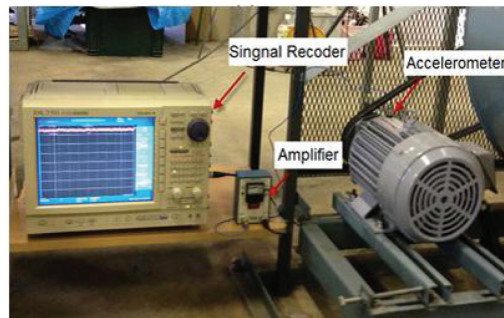
(b) JNU bearing test rig
