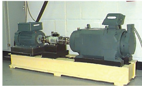
(a) CWRU bearing test rig
