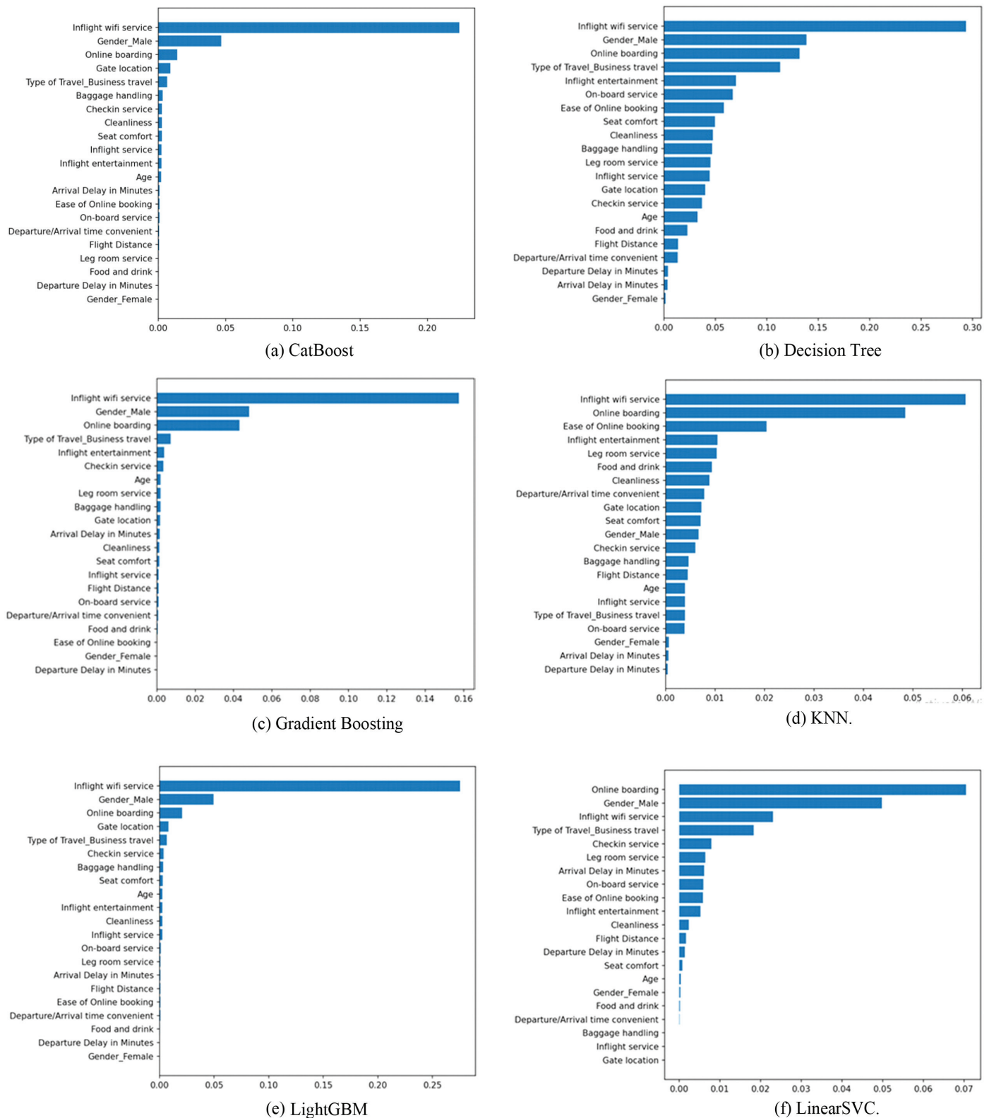
Fig. 1. Permutation importance across models (a–j): (a) CatBoost, (b) Decision Tree, (c) Gradient Boosting, (d) KNN, (e) LightGBM, (f) LinearSVC, (g) Logistic Regression, (h) Random Forest, (i) SGD, and (j) XGBoost.
