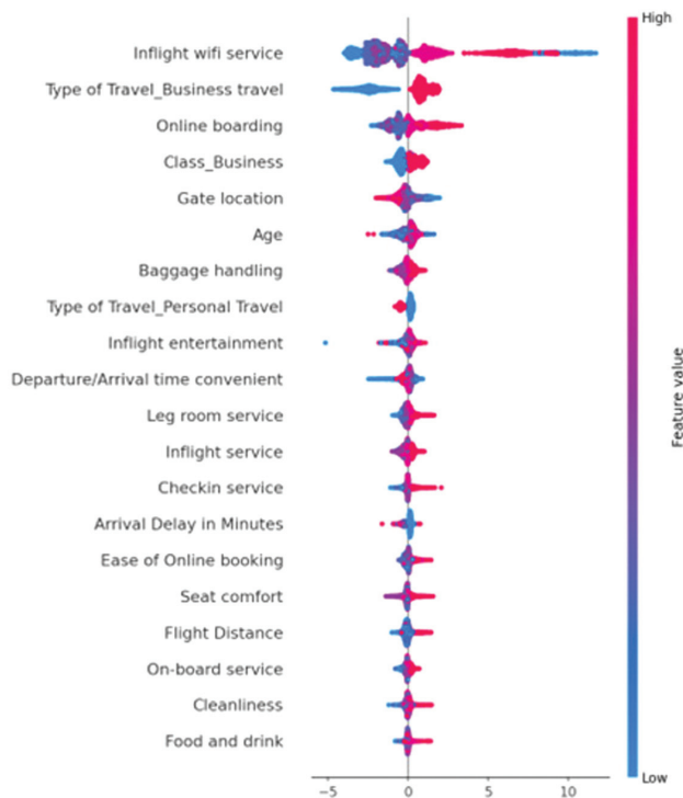
(g) SHAP beeswarm — LightGBM
