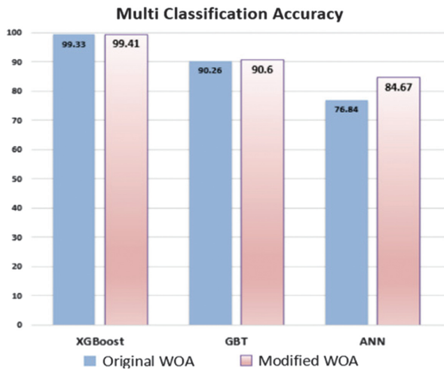
Fig. 21. Comparison of accuracy between the modified and original WOA (multiclass classification).
