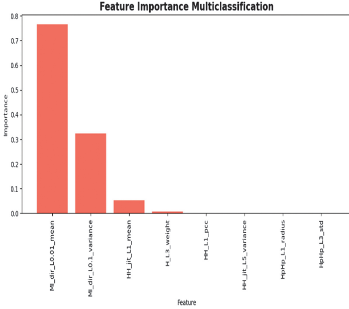
Fig. 9. Importance of the selected features (multiclass classification).
