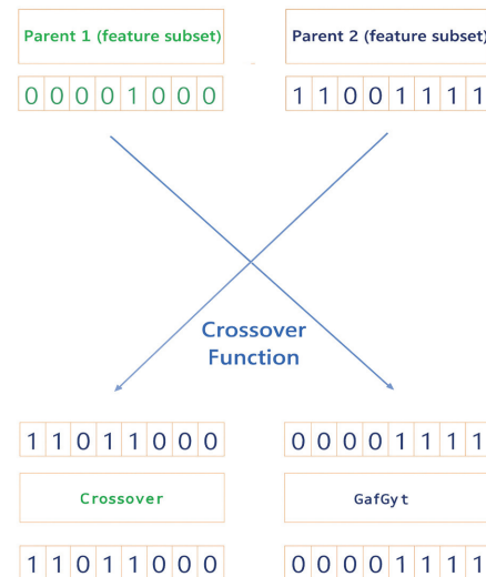
Fig. 5. Representation of the crossover process.
