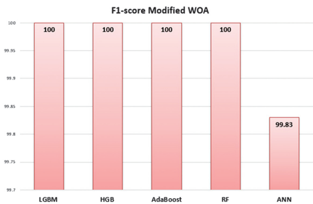
Fig. 12. Ranking of classifier in terms of f1-score (binary classification).
