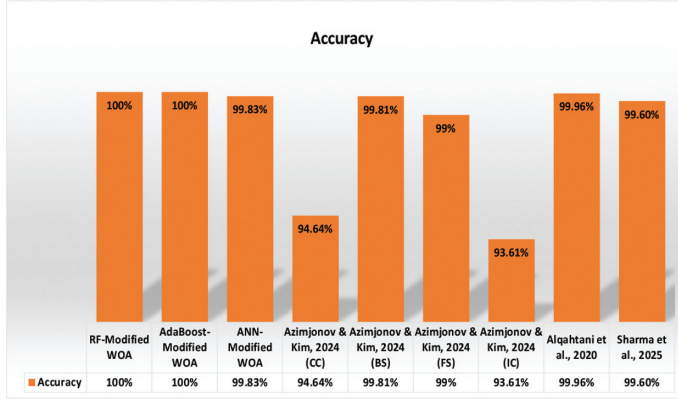
Fig. 25. Accuracy comparison between widely used baselines and the modified WOA.
