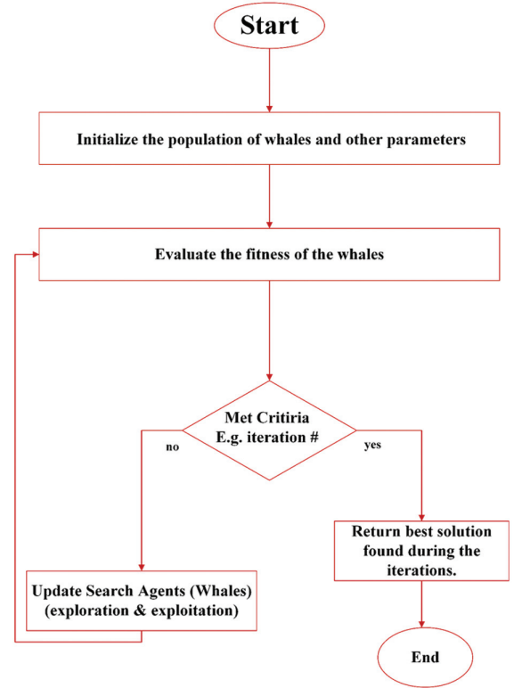
Fig. 2. Operations of the WOA algorithm.
