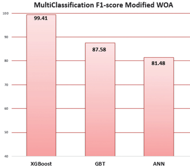
Fig. 16. Ranking of classifiers in terms of f1-score (multiclass classification).
