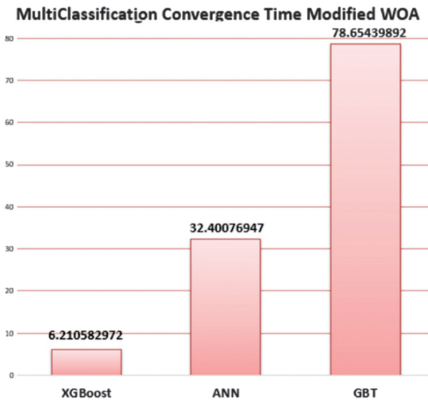
Fig. 17. Ranking of classifiers in terms of convergence time (multiclass classification).
