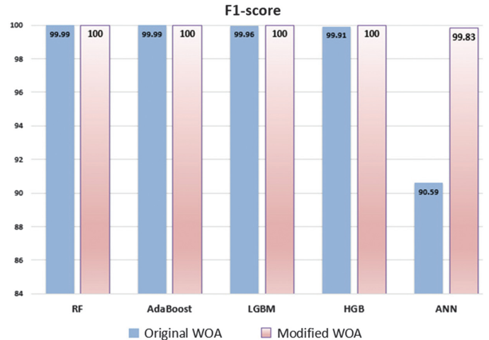
Fig. 20. Comparison of f1-score between the modified and original WOA (binary classification).
