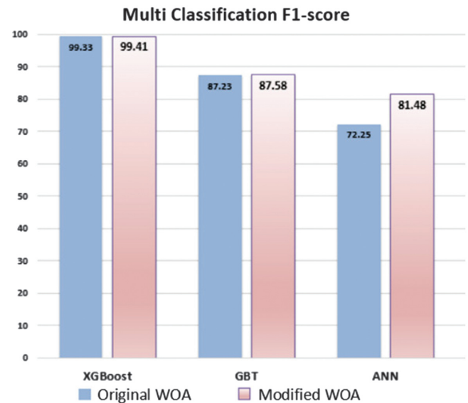
Fig. 23. Comparison of f1-score between the modified and original WOA (multiclass classification).
