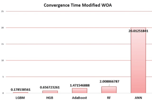
Fig. 13. Ranking of classifiers in terms of convergence time (binary classification).
