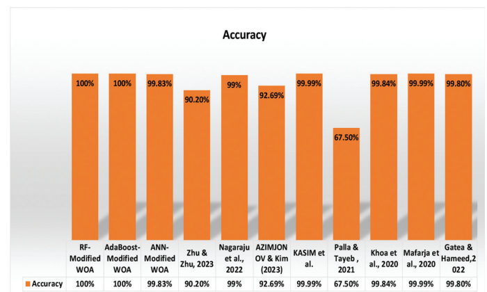
Fig. 24. Accuracy comparison between existing frameworks and the modified WOA.
