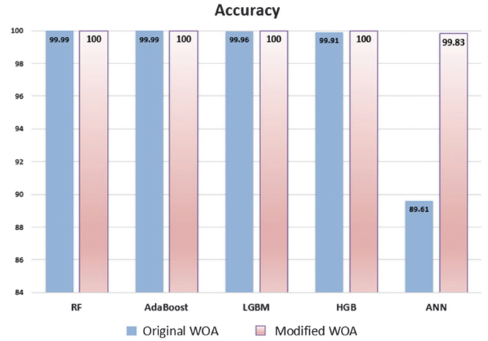
Fig. 18. Comparison of accuracy between the modified and original WOA (binary classification).
