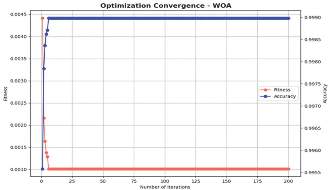
Fig. 6. Convergence plot of the WOA (binary classification).
