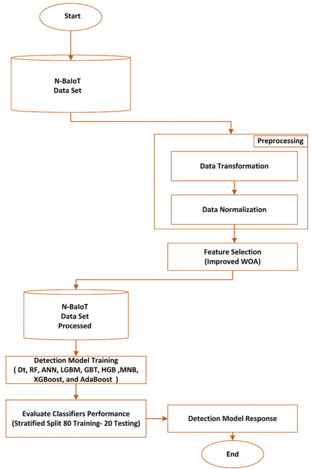
Fig. 3. Proposed ML-based IoT attack detection model.
