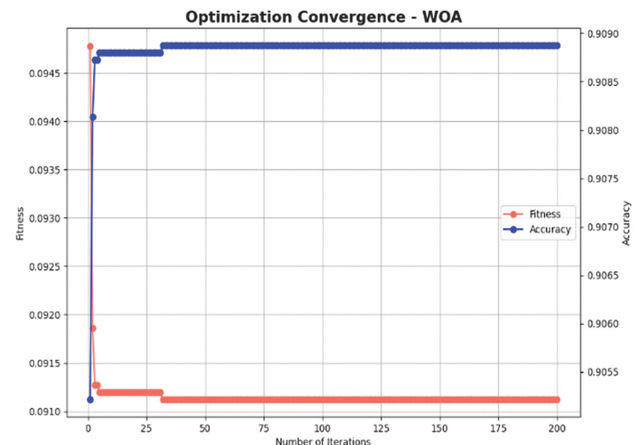
Fig. 8. Convergence plot of the WOA (multiclass classification).
