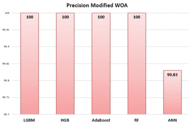
Fig. 11. Ranking of classifiers in terms of precision (binary classification).
