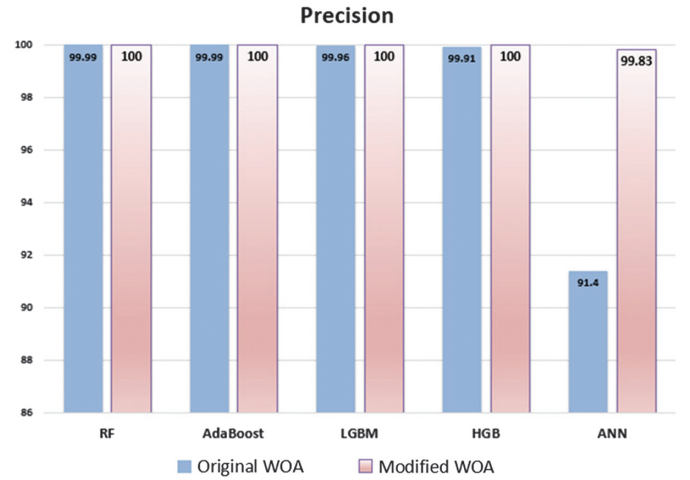
Fig. 19. Comparison of precision between the modified and original WOA (binary classification).
