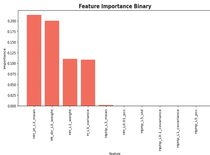
Fig. 7. Importance of the selected features (binary classification).
