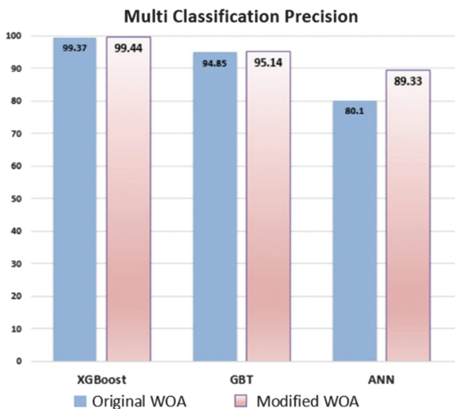
Fig. 22. Comparison of precision between the modified and original WOA (multiclass classification).
