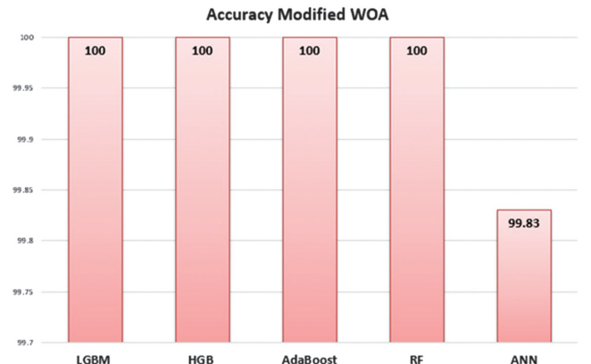
Fig. 10. Ranking of classifiers in terms of accuracy (binary classification).
