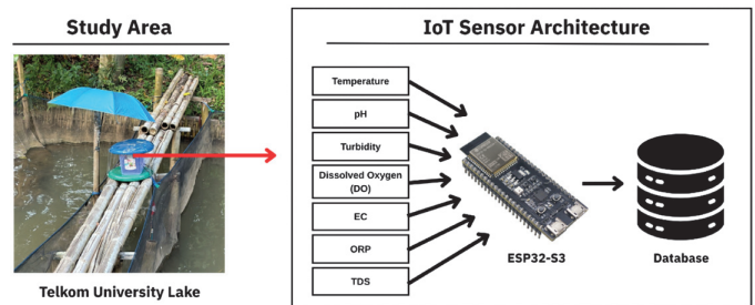
Fig. 2. Study area and IoT sensor architecture. Seven probes are read by an ESP32-S3 node and written to a database.
