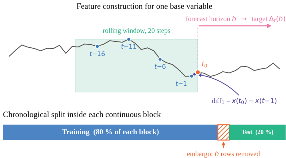
Fig. 5. Feature construction and leakage control. Upper panel: the features built from one base variable (one of the seven sensor channels or the index itself), showing the lags, the rolling window, the first difference, and the h -step target. Lower panel: chronological split within each continuous block, with an embargo of h rows at the test boundary.
