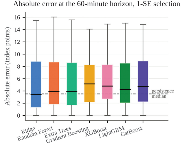
Fig. 7. Distribution of absolute error at the 60-min horizon under 1-SE selection. The dashed line marks the median absolute error of the persistence baseline on the same rows.
