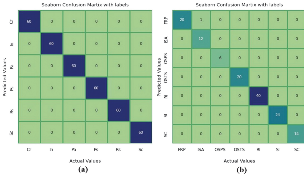
Fig. 6. (a) Confusion matrix of the proposed ensemble model for classification of the six types of hot-rolled steel surface defects on the NEU dataset. (b) Confusion matrix of the proposed ensemble model for classification of the seven types of hot-rolled steel surface defects on the X-SDD dataset.
