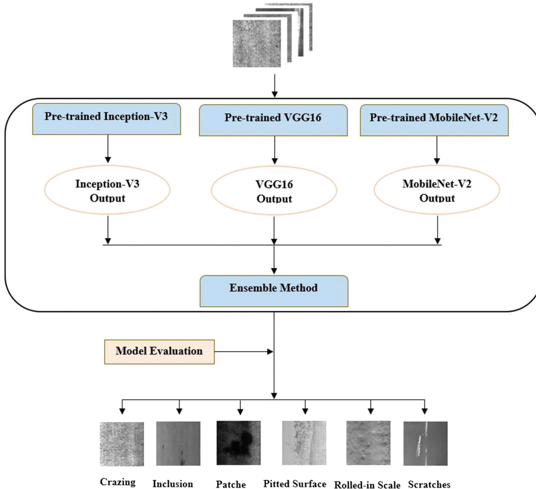
Fig. 1. Flow chart of the proposed ensemble model for steel surface defect classification.
