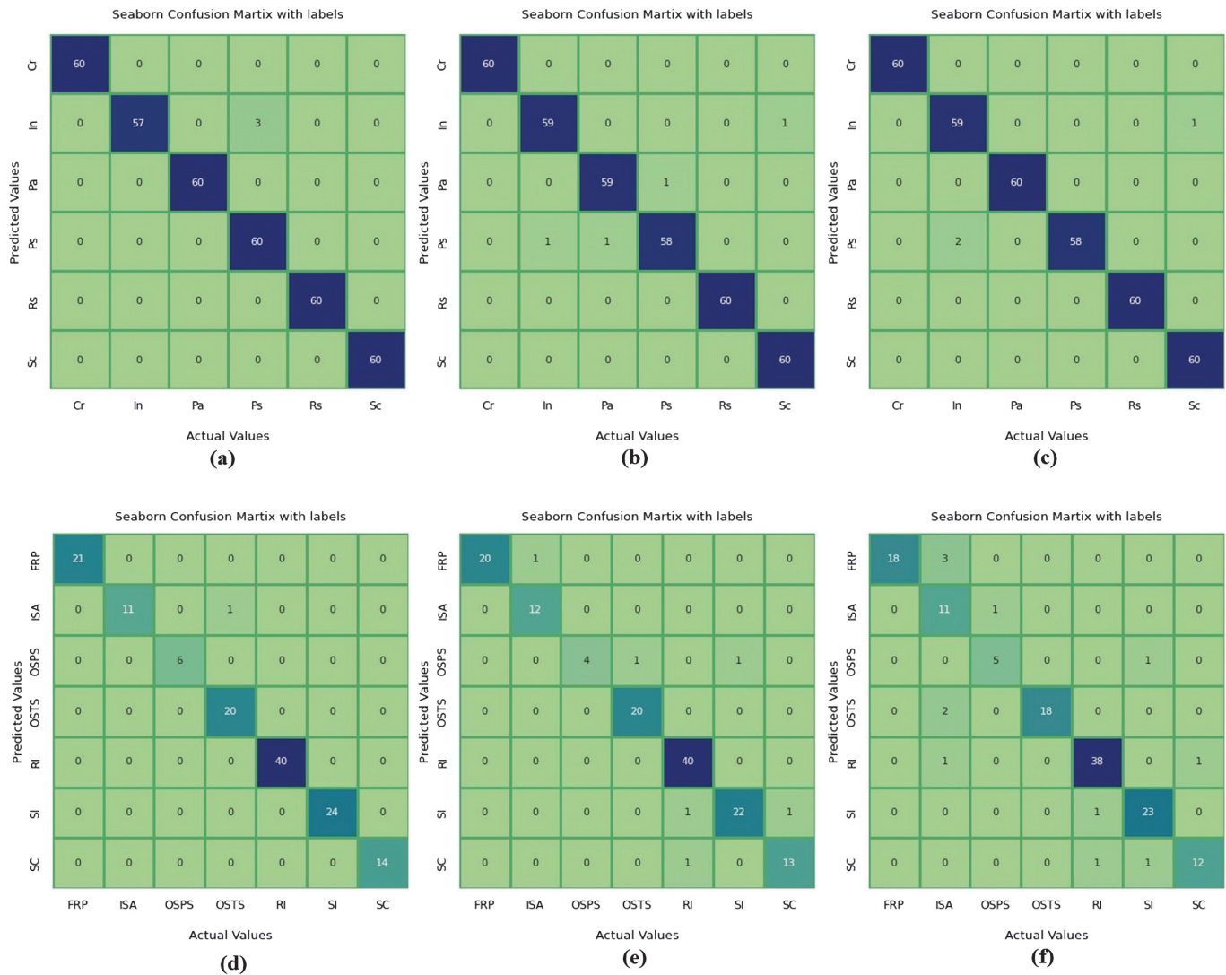
Fig. 4. (Top) Confusion matrix of base models for classification of the six types of hot-rolled steel surface defects on the NEU dataset: (a) Inception-V3, (b) VGG16, (c) MobilNet. (Down) Confusion matrix of base models for classification of the seven types of hot-rolled steel surface defects on the X-SDD dataset: (d) Inception-V3, (e) VGG16, (f) MobilNet.
