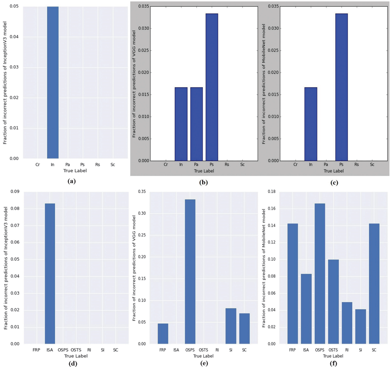
Fig. 5. (Top) Fraction of incorrect predictions of the base models for classification of the six types of hot-rolled steel surface defects on the NEU dataset: (a) Inception-V3, (b) VGG16, (c) MobilNet. (Down) Fraction of incorrect predictions for seven types of hot-rolled steel surface defects on the X-SDD dataset: (d) Inception-V3, (e) VGG16, (f) MobilNet.
