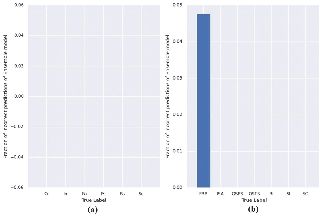
Fig. 7. (a) Fraction of incorrect predictions of the proposed ensemble model for classification of the six types of hot-rolled steel surface defects on the NEU dataset. (b) Fraction of incorrect predictions of the proposed ensemble model for classification of the seven types of hot-rolled steel surface defects on the X-SDD dataset.
