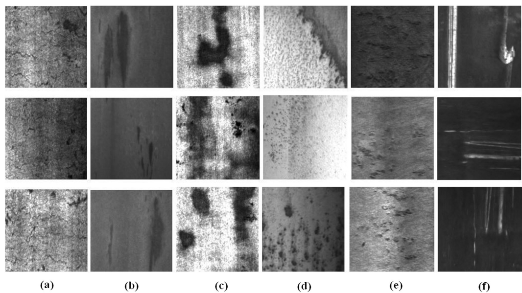
Fig. 2. Samples for the six kinds of defect classes of the NEU dataset including (a) crazing (Cr), (b) inclusion (In), (c) patches (Pa), (d) pitted surface (Ps), (e) rolled-in scale (Rs), (f) scratches (Sc).
