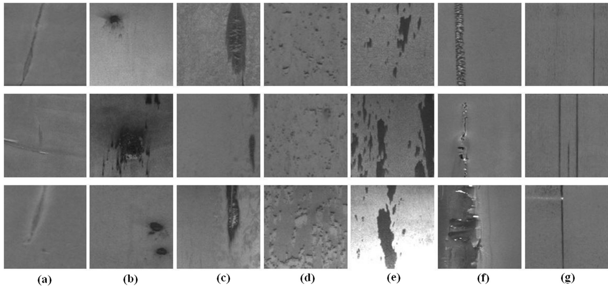
Fig. 3. Samples for the seven kinds of defect classes of the X-SSD dataset including (a) finishing roll printing (Fr), (b) iron sheet ash (Is), (c) oxide scale-of-plate system (Op), (d) oxide scale-of-temperature system (Ot), (e) red iron sheet (Ri), (f) inclusion (Si), (g) scratches (Ss).
