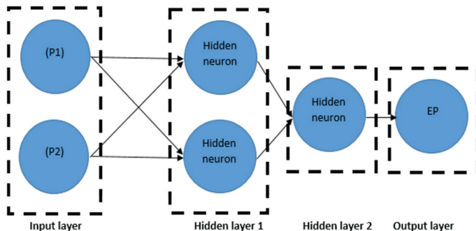
Fig. 5. ANN structure model for two input parameters (P1+P2).
